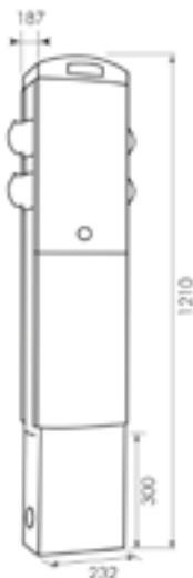
Version tranchee
